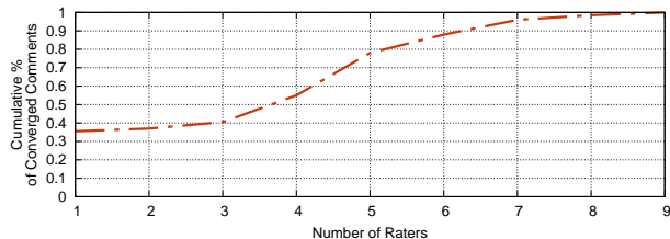
Figure 1: Toxicity Convergence —We observe an inflection point where after five participants rate a comment, the benefit of additional perspectives falls off.
